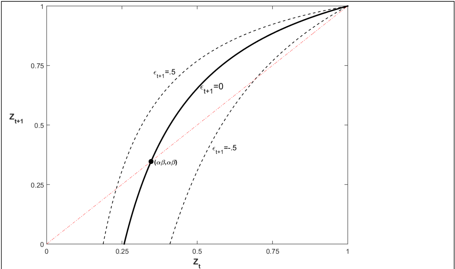
Fig.1. Long & Plosser model: investment/output ratio at t+1, Z_{t+1} , as a function of Z_t for
